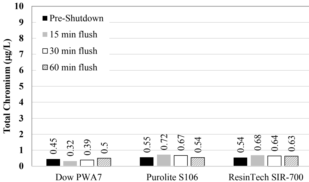
Figure A.11 Total chromium leaching after 4-hour shutdown
