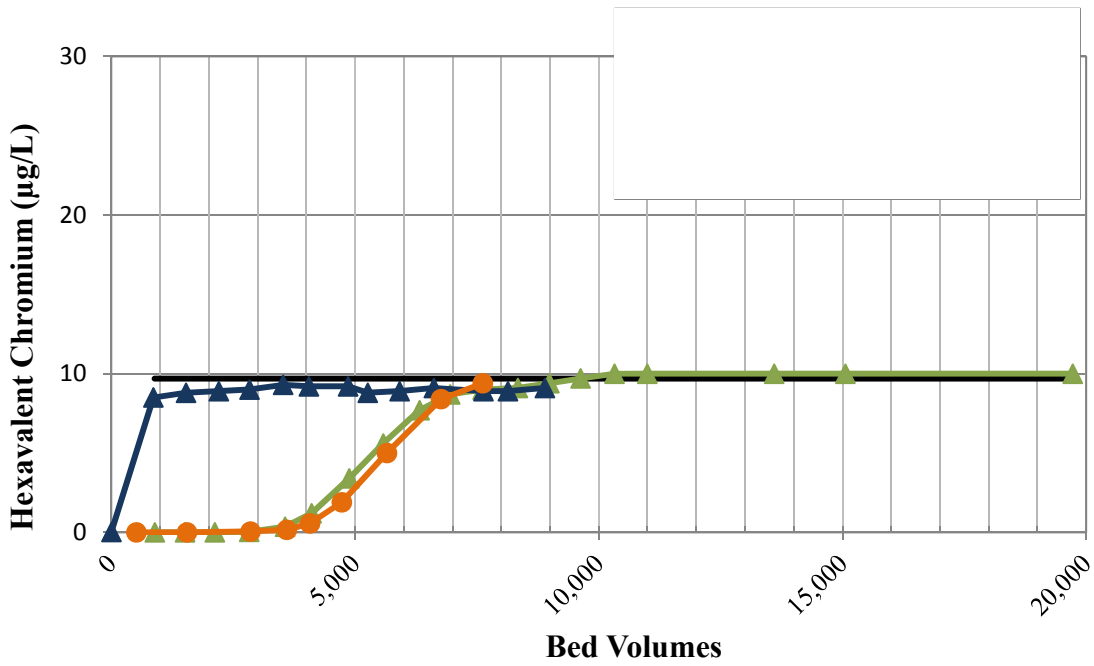
Figure 3.3 Cr(VI) breakthrough for SBA Resins at Livermore
