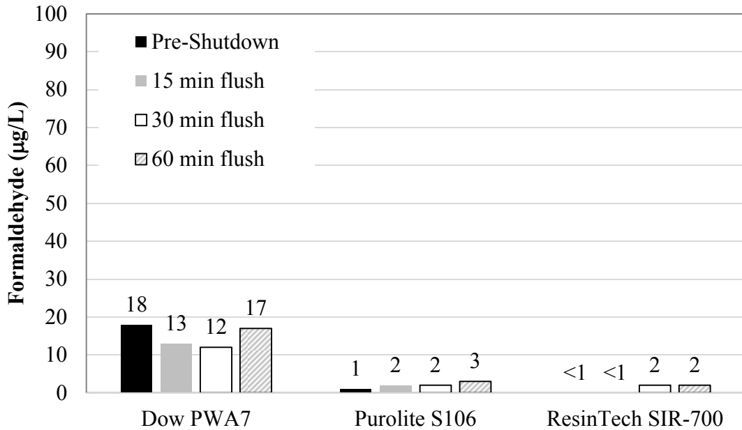
Figure A.6 Formaldehyde leaching after 72-hour shutdown
