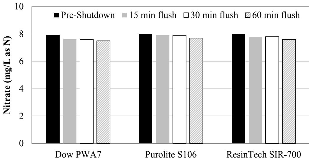
Figure A.7 Nitrate leaching after 72-hour shutdown
