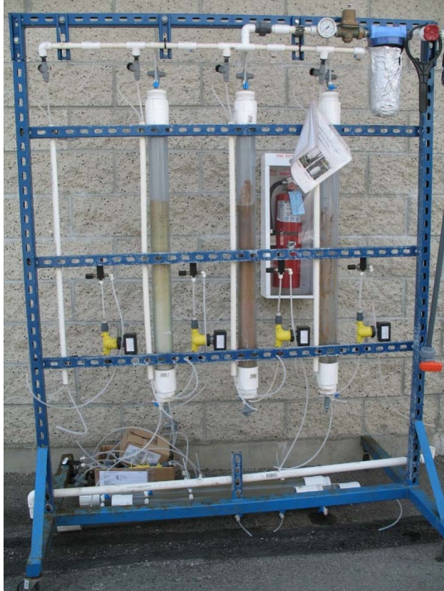
Figure 2.2 Photograph of an example ion exchange pilot unit
