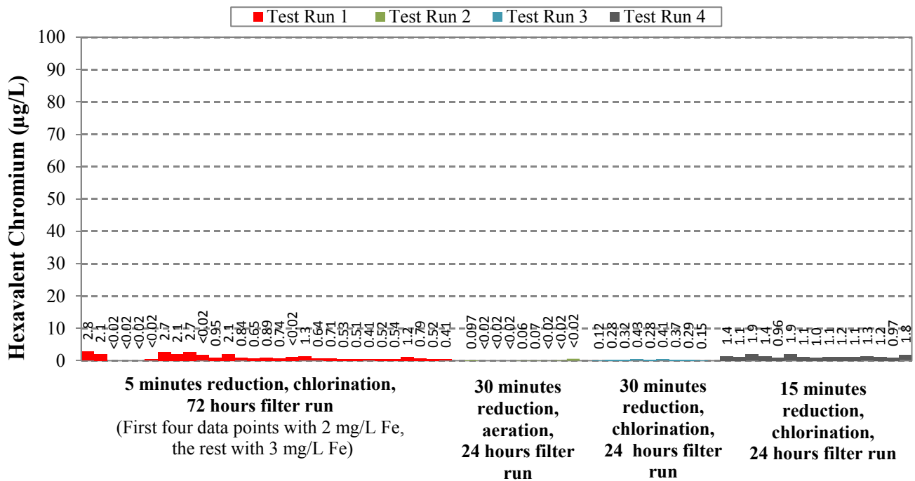
Figure 4.2 RCF post-reduction Cr(VI) with various reduction times and chlorination
