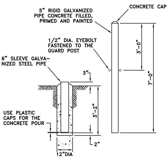
REMOVABLE BARRIER POST DETAIL
