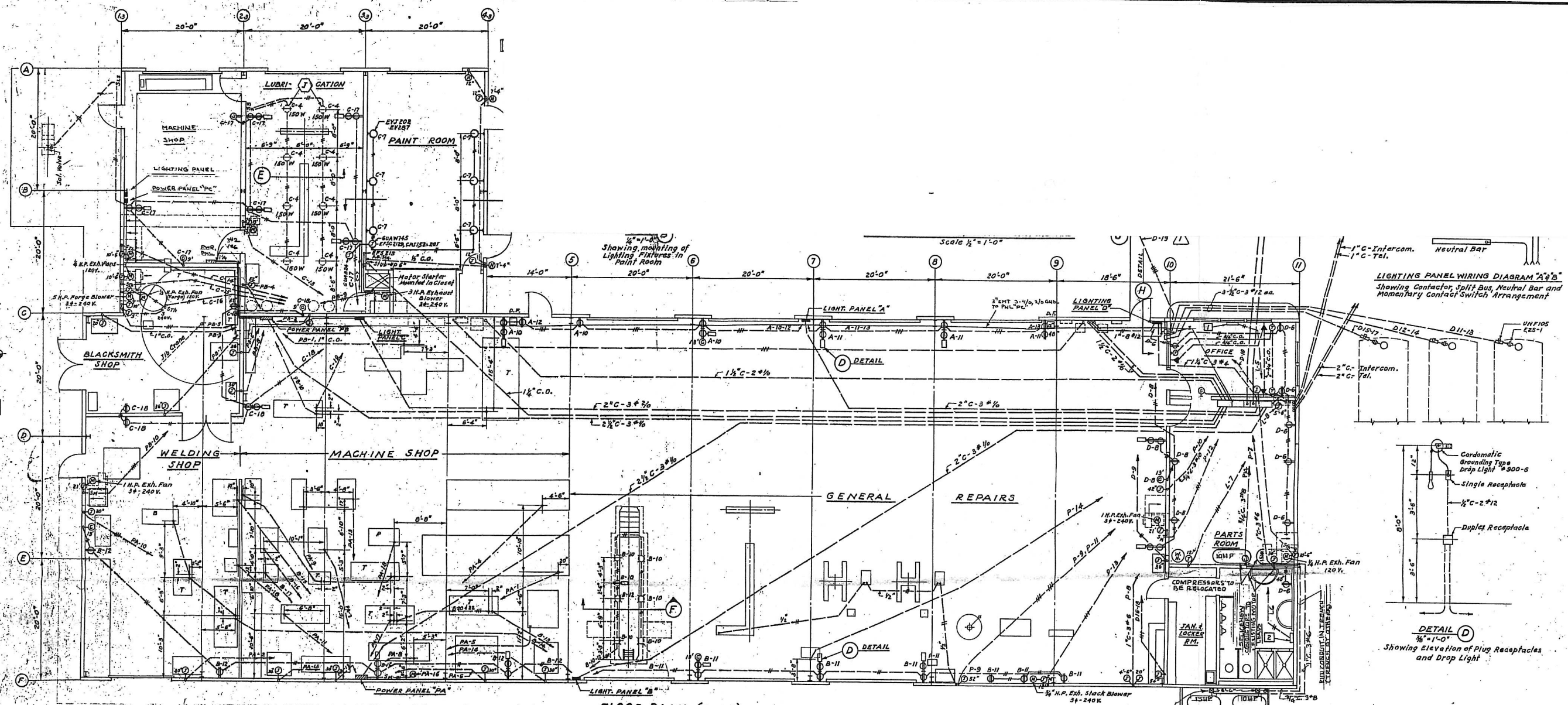
FLOOR PLAN (POWER) Scale 1/8" = 1'-0"
